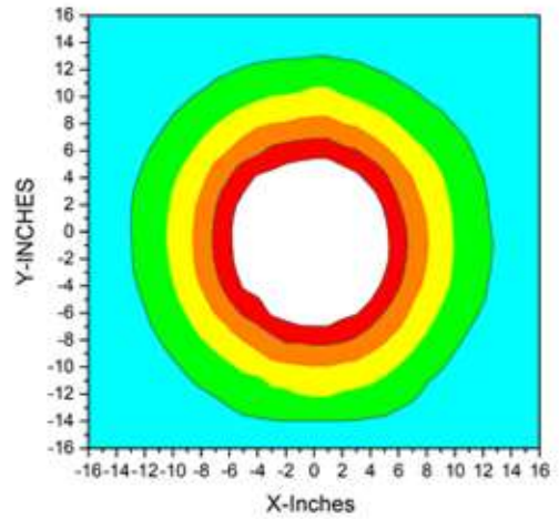
Beam Irradiance Profile for EDG-4W at 4 Feet (122cm)
