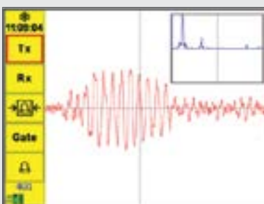
RF (A-Scan Waveform) with Frequency Spectrum Inset
