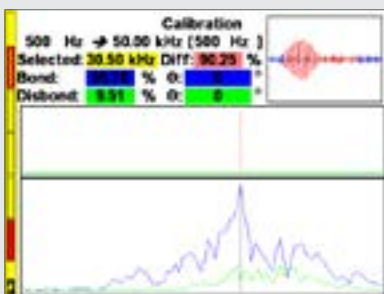
Pitch-Catch Mode calibration showing the bond and dis-bond spectrum.
