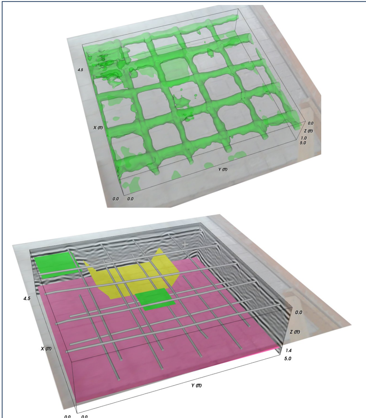
Figure 8. Scan results from the concrete test wall built by Olson Engineering (Wheat Ridge, CO) with the quickly generated isosurface view (top). More subtle features in the radar images can be found by examining the cross-section images in the 2D and 3D views, and then creating targets (bottom). Rebar are shown in gray, the void and honeycomb regions in green, the weak zone in yellow, and the slab bottom in pink.
