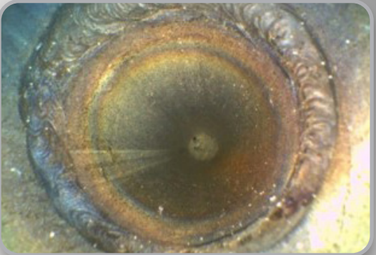
Orbital Weld
