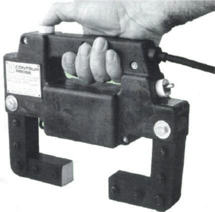
DA-200 Contour Probe (115 VAC) Federal Stock No. 0635-00-022-0372 DA-200S Contour Probe (230 VAC, 50 Hz) Federal Stock No. 0635-01-073-0844
