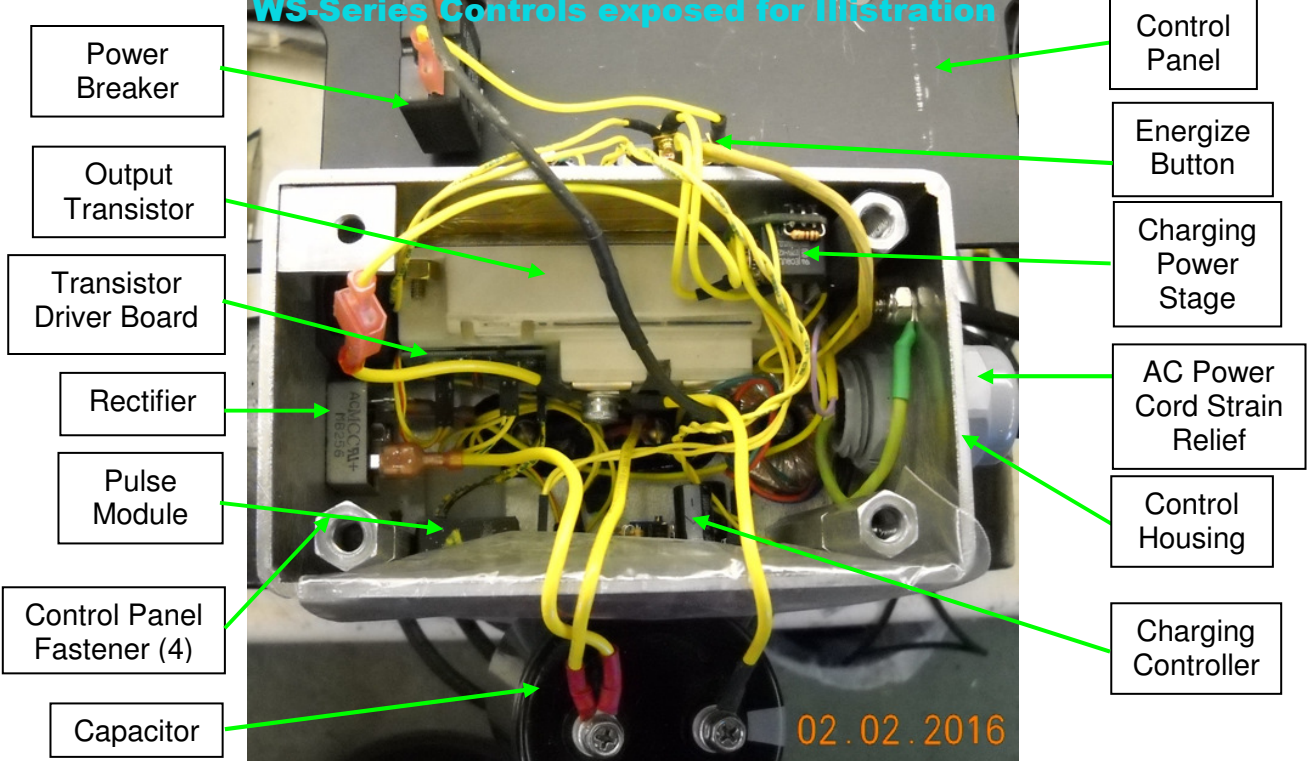
WS-Series Controls exposed for illustration
