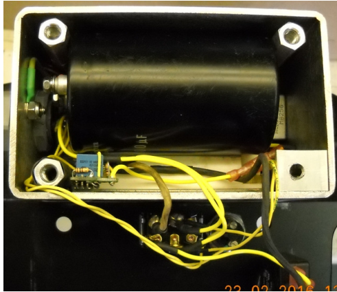
WS-Series Controls exposed for illustration
