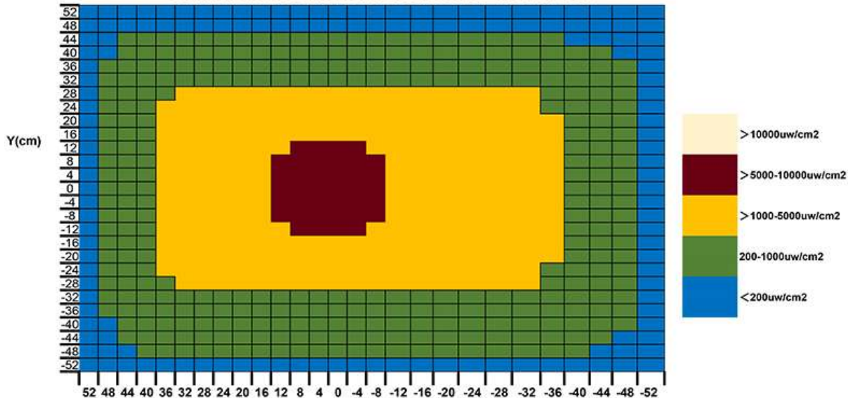
BEAM IRRADIANCE PROFILE AT 38CM FOR LW-365 & LW-365V
