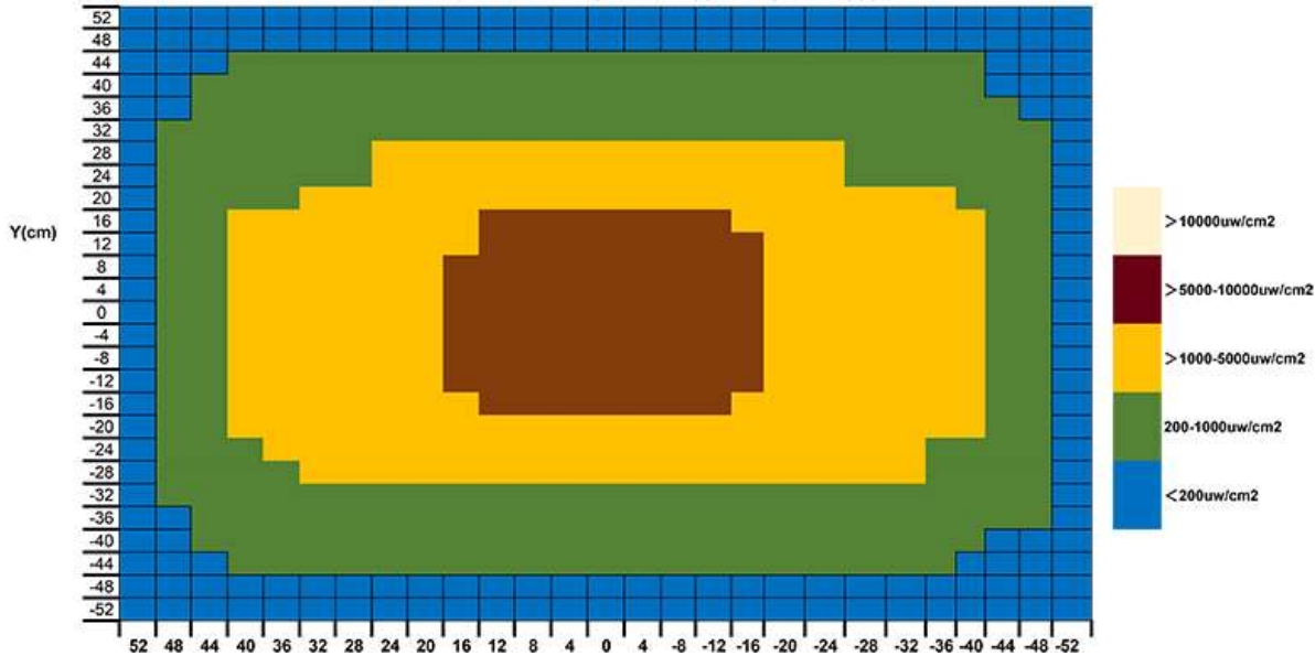
BEAM IRRADIANCE PROFILE AT 38CM FOR LW-365L
