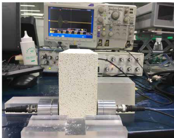
Experiment of 250KHz air-coupled probe penetrating 64mm refractory brick
