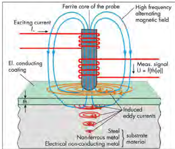
Schematic diagram of the phase sensitive eddy current method. The indentation depth of the magnetic field depends on the used frequency and the electrical conductivity of the materials.
