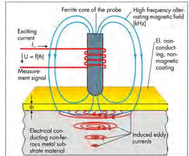
Schematic diagram of the amplitude sensitive eddy current test method. The indentation depth depends on the used frequency and the electrical conductivity of the substrate material.
