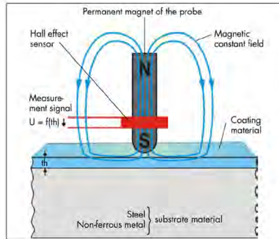
Schematic diagram of the magnetic test method. The indentation depth of the magnetic field depends on the permeability of the substrate material.
