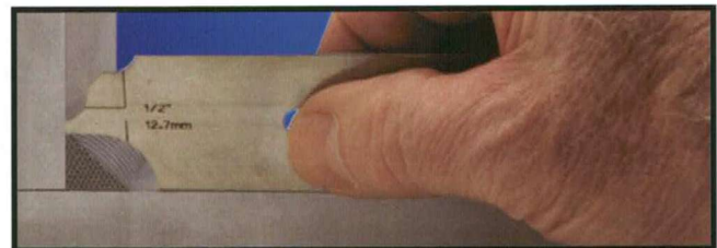
CHECKING FILLET LEG SIZE
