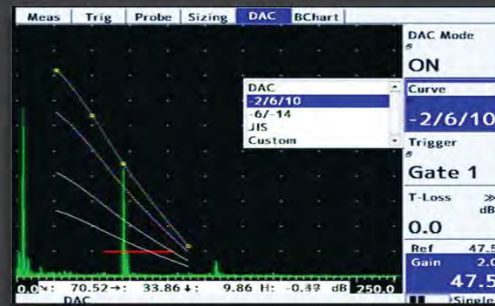
Library of DAC Curves
