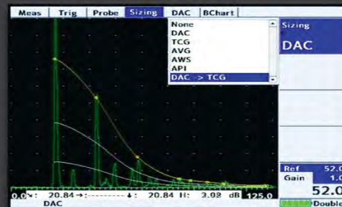
DAC to TCG conversion
