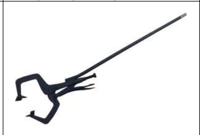
IRWIN VISE-GRIP C Clamp (11R) with Welded Angle Iron and an 18" CS Rod Welded
