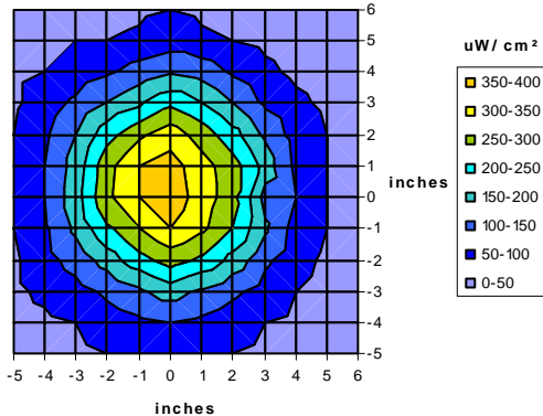
XeLED-Ni1UV-R3-365-M intensity at 15"
