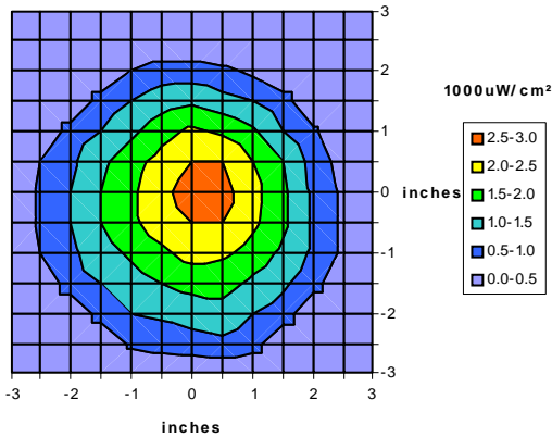
XeLED-Ni1UV-R-365-SS intensity at 15"
