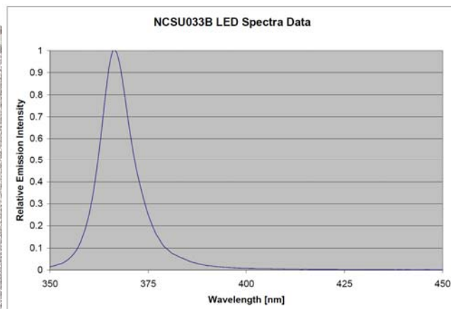
Spectra shows true 365nm UVA emission!
